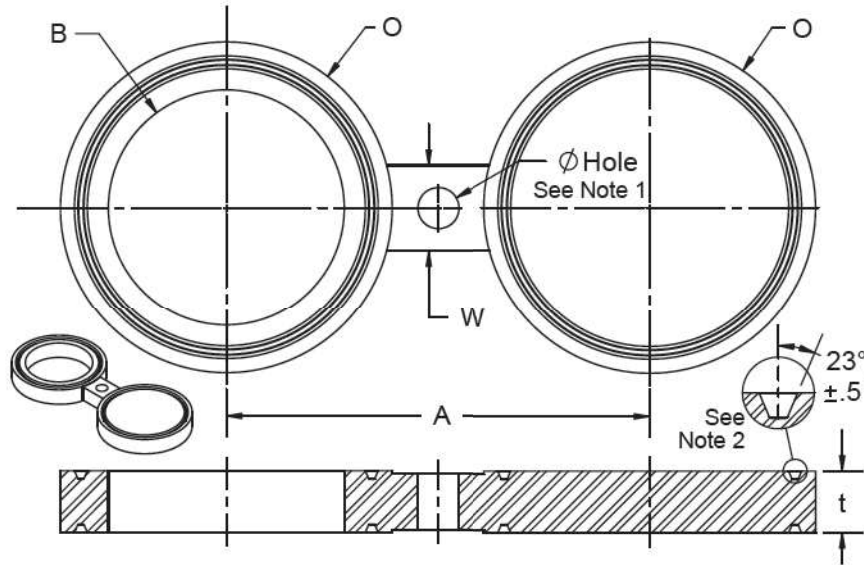
Dimensions of Class 2500 Female Ring-Joint Facing Figure 8 Blanks
