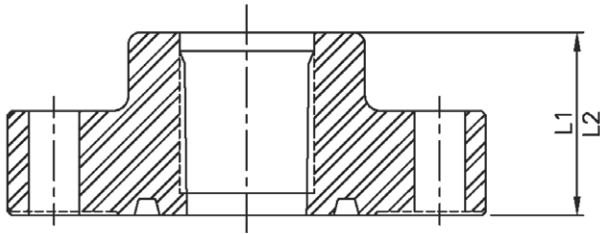
THREADED FLANGE
